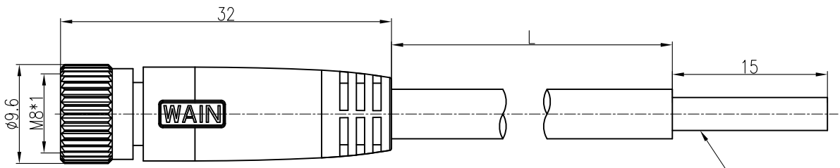
剥线长度 Stripping length of the sheath
