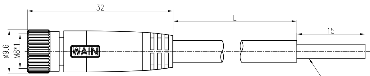
剥线长度 Stripping length of the sheath
