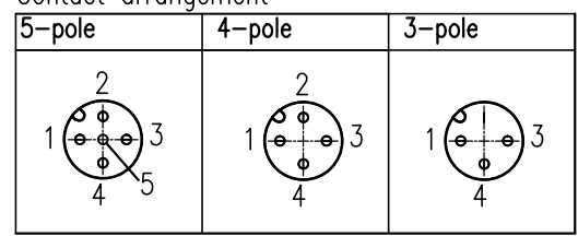
针位排布图 Contact arrangement
