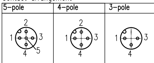
Contact arrangement
