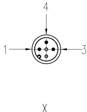
针位图 Contact arrangement
