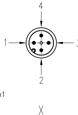
针位图 Contact arrangement
