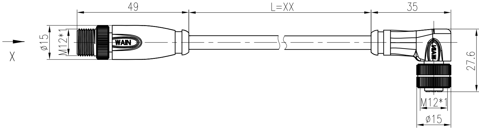
针位图 Contact arrangement
