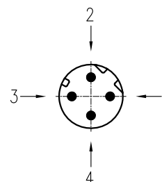
针位图 Contact arrangements
