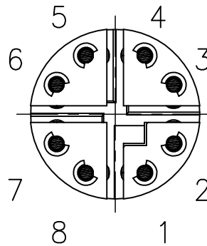
针位图 Contact arrangements
