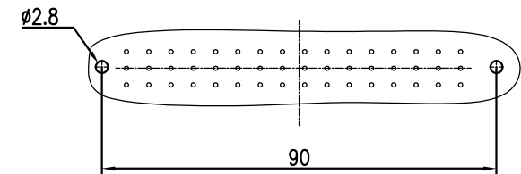
面板安装开孔图 Panel cut out
